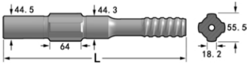
Gardner-Denver PR 123
